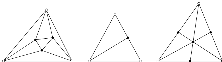
FIGURE 5.1. Subdivisions of a 2-simplex
