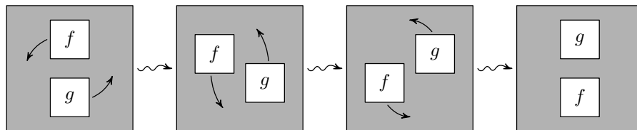
FIGURE 3.3. Commutativity of the product operation
