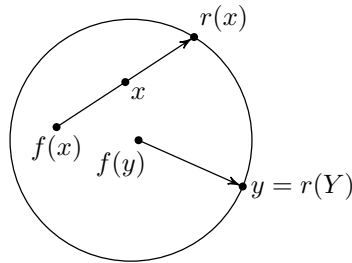
FIGURE 1. Proof of Brouwer's Theorem
