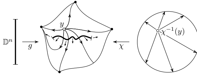
FIGURE 2. Blowing out the image of g
